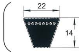
C CLASSICAL v-belt
