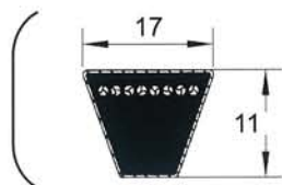
B CLASSICAL v-belt
