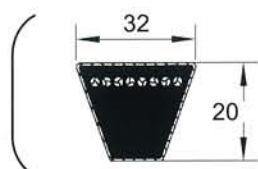
D CLASSICAL v-belt
