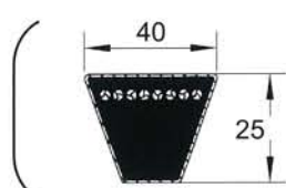
E CLASSICAL v-belt
