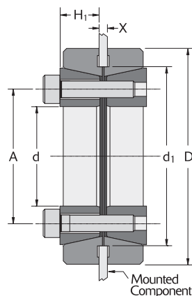
Base Part Number d (inch) D (inch) H 1 (inch) A (inch) d 1 (inch) Locking Screws Mounted Component Thickness (X) M a M t Th P s Ship Weight (lb) Range 1 Range 2 Maximum Transmitted Qty Size X (inch) Screw Length 1 (mm) X (inch) Screw Length 2 (mm) Install Torque (ft lb) Torque (ft lb) Thrust (lbs) BCH502008 1/2 1.85 0.384 0.984 1.457 5 M5 0.098 – 0.197 20 0.197 – 0.394 25 7 104 4970 42.5 0.7 BCH502010 5/8 1.85 0.384 0.984 1.457 5 M5 0.098 – 0.197 20 0.197 – 0.394 25 7 129 5510 33.9 0.4 BCH502012 3/4 2.047 0.384 1.181 1.654 6 M5 0.098 – 0.197 20 0.197 – 0.394 25 7 186 6610 33.9 0.7 BCH502014 7/8 2.283 0.463 1.398 1.890 6 M5 0.098 – 0.315 25 0.315 – 0.512 30 7 217 6610 24.2 0.9 BCH502015 15/16 2.283 0.463 1.398 1.890 6 M5 0.098 – 0.315 25 0.315 – 0.512 30 7 233 6610 22.6 0.9 BCH502100 1 2.283 0.463 1.398 1.890 6 M5 0.098 – 0.315 25 0.315 – 0.512 30 7 248 6610 21.2 0.9 BCH502102 1 1/8 2.559 0.463 1.594 2.126 8 M5 0.098 – 0.315 25 0.315 – 0.512 30 7 385 9130 26.0 1.1 BCH502103 1 3/16 2.559 0.463 1.594 2.126 8 M5 0.098 – 0.315 25 0.315 – 0.512 30 7 406 9130 24.7 1.1 BCH502104 1 1/4 2.953 0.561 1.850 2.362 8 M6 0.098 – 0.350 30 0.350 – 0.547 35 12 564 12030 26.5 1.8 BCH502106 1 3/8 2.953 0.561 1.850 2.362 8 M6 0.098 – 0.350 30 0.350 – 0.547 35 12 621 12030 24.1 1.8 BCH502107 1 7/16 3.307 0.561 2.047 2.598 10 M6 0.098 – 0.350 30 0.350 – 0.547 35 12 811 15040 28.7 2.2 BCH502108 1 1/2 3.307 0.561 2.047 2.598 10 M6 0.098 – 0.350 30 0.350 – 0.547 35 12 846 15040 27.6 2.2 BCH502110 1 5/8 3.78 0.699 2.362 2.992 7 M8 0.098 – 0.323 35 0.323 – 0.630 45 30 1261 20710 28.0 3.5 BCH502111 1 11/16 3.78 0.699 2.362 2.992 7 M8 0.098 – 0.323 35 0.323 – 0.630 45 30 1310 20710 27.0 3.5 BCH502112 1 3/4 3.78 0.699 2.362 2.992 7 M8 0.098 – 0.323 35 0.323 – 0.630 45 30 1358 20710 26.0 3.5 BCH502114 1 7/8 4.528 0.699 2.756 3.386 8 M8 0.098 – 0.323 35 0.323 – 0.630 45 30 1663 23650 27.7 5.3 BCH502115 1 15/16 4.528 0.699 2.756 3.386 8 M8 0.098 – 0.323 35 0.323 – 0.630 45 30 1719 23650 26.8 5.1 BCH502200 2 4.528 0.699 2.756 3.386 8 M8 0.098 – 0.323 35 0.323 – 0.630 45 30 1774 23650 26.0 5.1 BCH502202 2 1/8 4.528 0.699 2.756 3.386 8 M8 0.098 – 0.323 35 0.323 – 0.630 45 30 1885 23650 24.5 4.9 BCH502203 2 3/16 4.528 0.699 2.756 3.386 8 M8 0.098 – 0.323 35 0.323 – 0.630 45 30 1940 23650 23.8 4.9 BCH502204 2 1/4 5.433 0.797 3.268 4.016 8 M10 0.098 – 0.335 40 0.335 – 0.630 50 60 3198 37900 32.5 8.6 BCH502206 2 3/8 5.433 0.797 3.268 4.016 8 M10 0.098 – 0.335 40 0.335 – 0.630 50 60 3375 37900 30.7 8.4 BCH502207 2 7/16 5.433 0.797 3.268 4.016 8 M10 0.098 – 0.335 40 0.335 – 0.630
