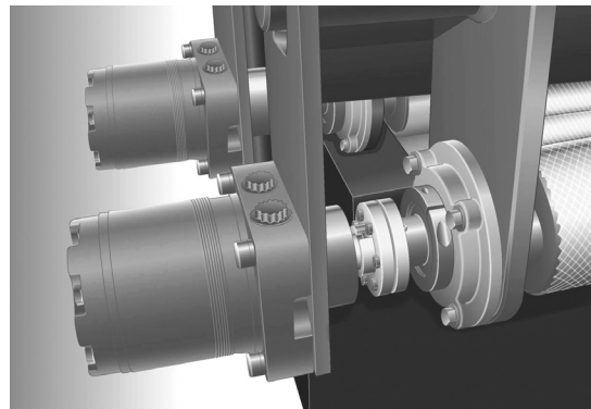
B-LOC Shrink Discs and WK Series Rigid Couplings facilitate torque-arm mounting of hydraulic drives directly onto the driven shaft, eliminating more expensive and less reliable flexible coupling arrangements.
