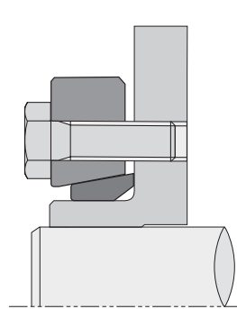
Half Shrink Disc Type HC
