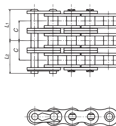
Triple strand
