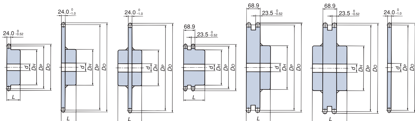
Mechanically machined 1B type
