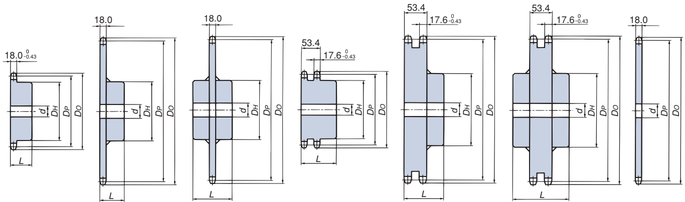
Mechanically machined 1B type Welded construction
