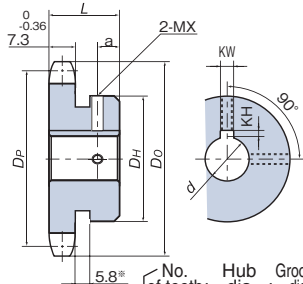
Hub with groove (9T – 12T)
