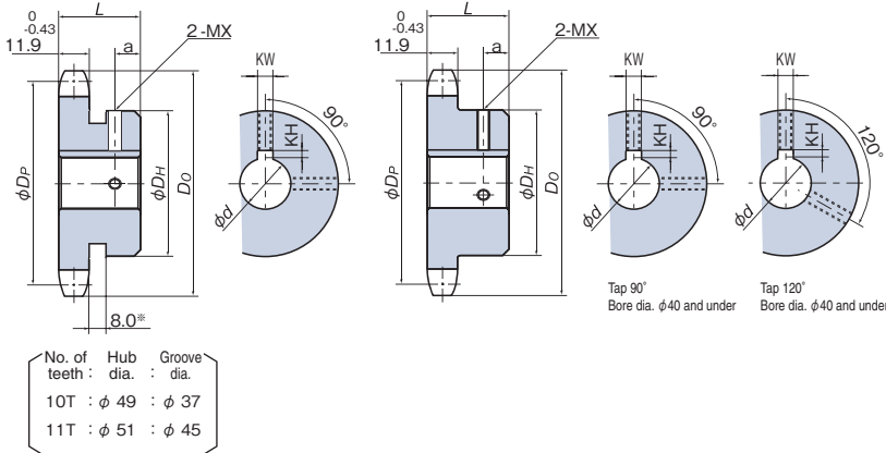
Hub with groove (10T – 11T)
