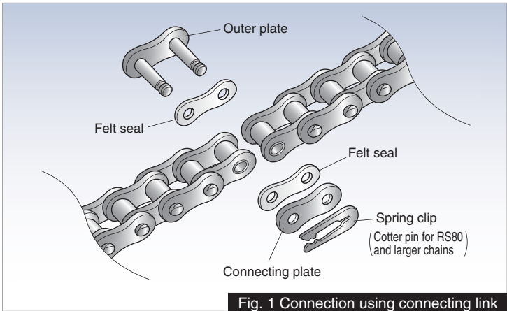
Fig. 1 Connection using connecting link
