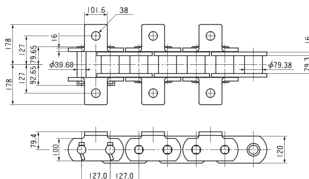
RS400-T-K1 Attachment Chain
