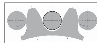
Unique Pin Gear Unit Tooth Profile
