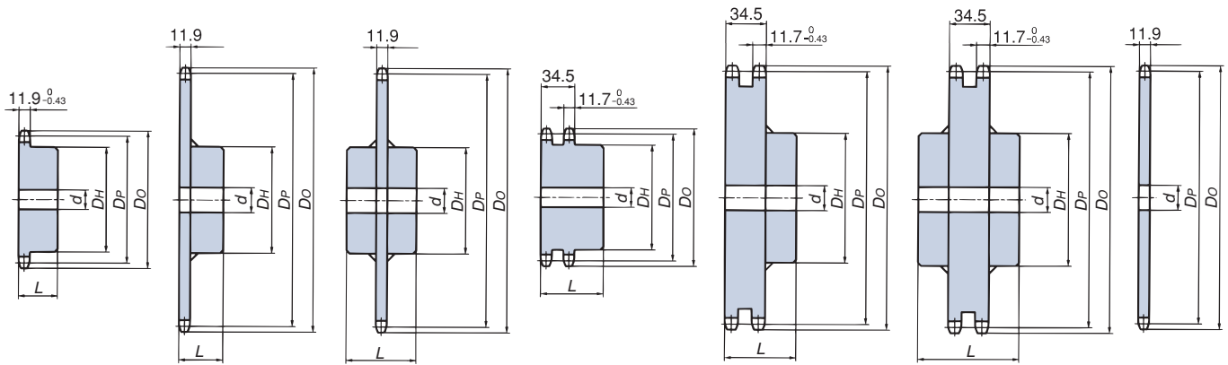
Mechanically machined 1B type
