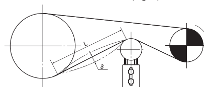
Fig. 7 Tensioner's anchored position
