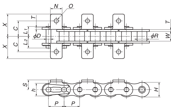
K1 Attachment
