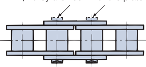
Fig. 1 Rivet-type roller chain
