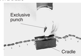
Fig. 7 Cutting Poly Steel Chain
