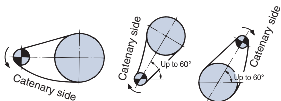
Fig. 18 General layout
