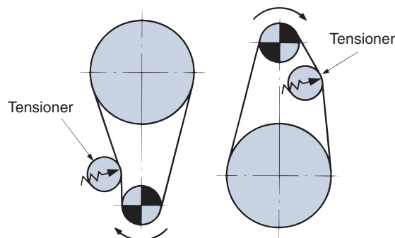
Fig. 22 Vertical transmission
