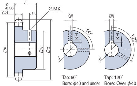
Hub without groove (13T and over)
