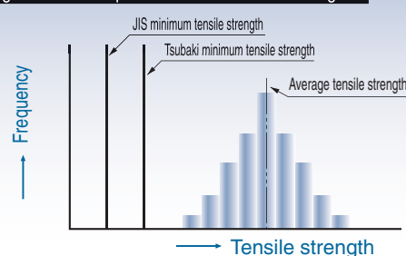
Fig. 1 Relationship between three tensile strengths
