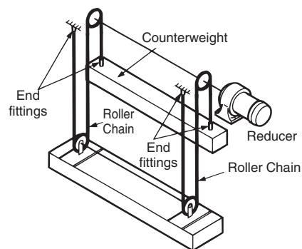
Lifting equipment (1)
