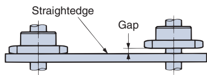
Fig. 17 Sprocket misalignment
