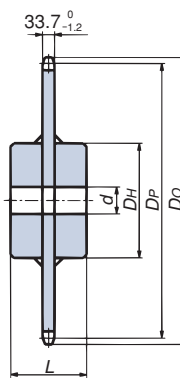
Welded construction 1C type
