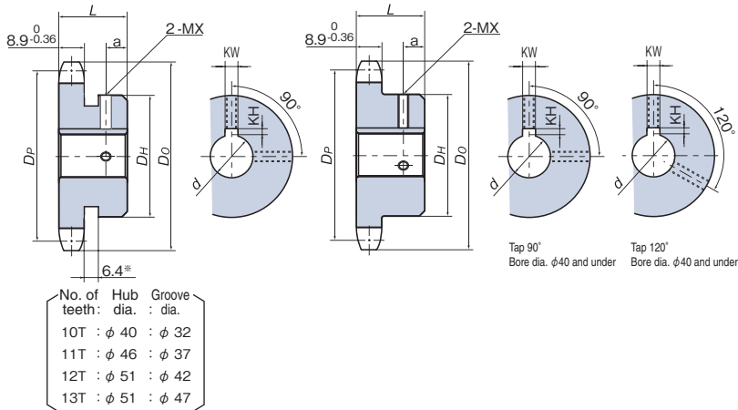
Hub with groove (10T – 13T)
