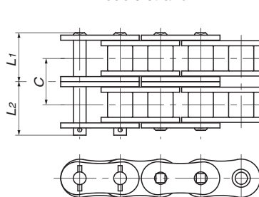
Double strand
