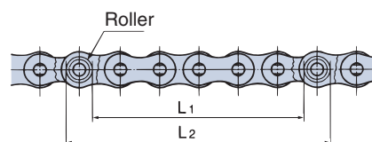
Fig. 28 Measuring length
