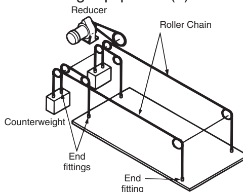
Lifting equipment (3)
