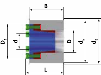
Mounting arrangement 2
