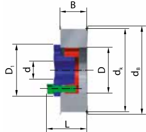
Mounting arrangement 1
