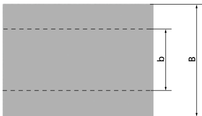
Tension plate variant A type 1
