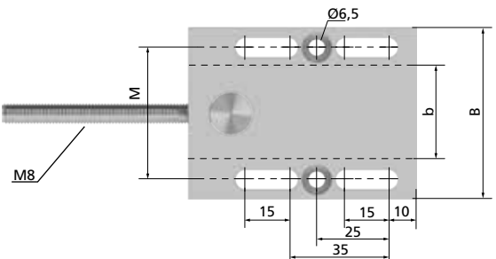
Tension plate variant A type 2
