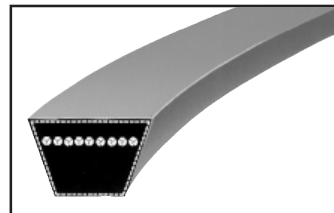
optibelt VB Classical belts to BS 3790 and DIN 2215
