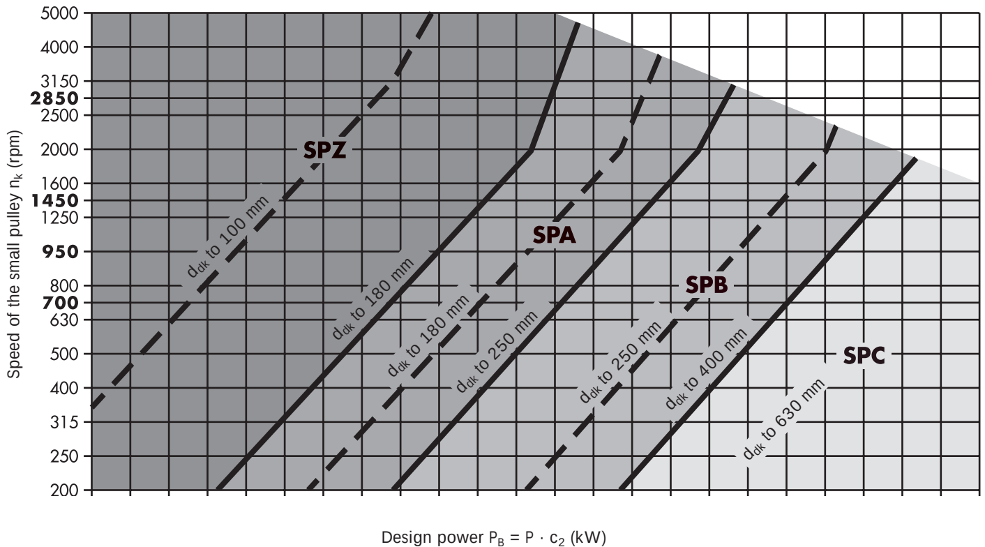
Diagram 2: Optibelt SK wedge belts to BS 3790/DIN 7753 Part 1
