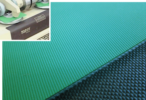
Y1 soft rough pattern and TABER comparative test machine.
